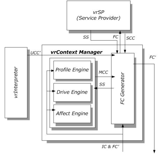
Figure 8: vrContextManager (vrCM).
