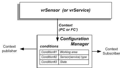
Figure 4: Configuration Manager.
