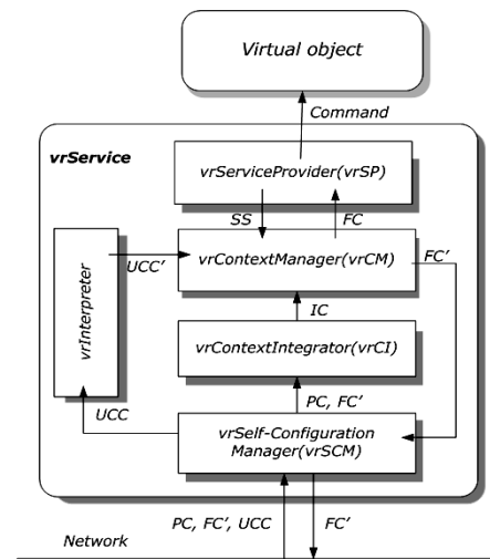
Figure 6: vrService components.
