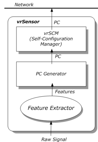
Figure 2: vrSensor.
