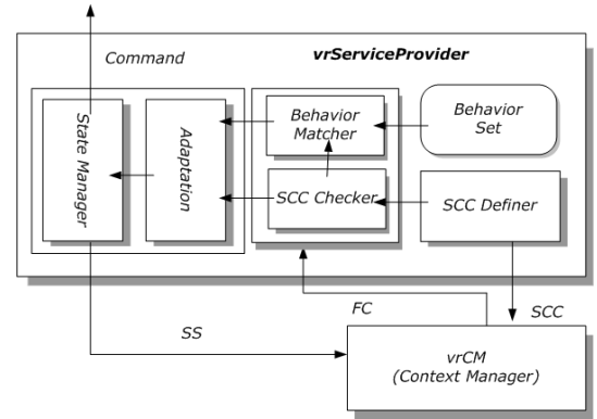
Figure 9: vrServiceProvider (vrSP).
