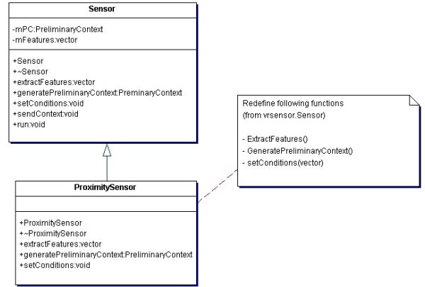
Figure 12: Implementation of ProximitySensor by using vrSensor .
